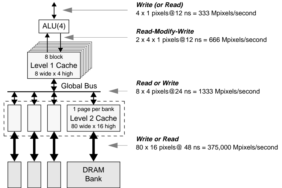
Figure 3-5 A logical representation of a Creator3D's four-way horizontally-interleaved frame buffer composed of twelve 3D-RAMs
