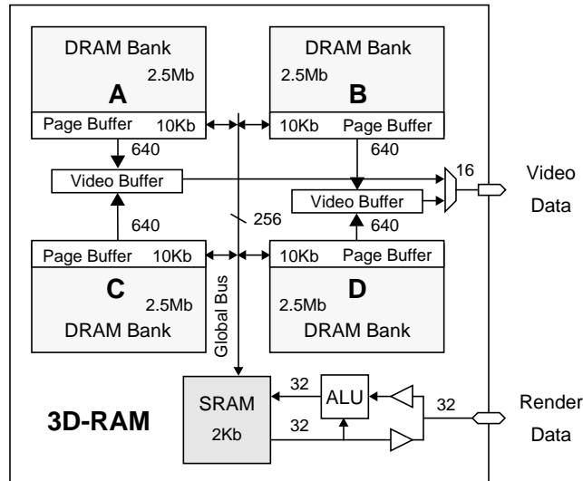
Figure 3-4 Internal block diagram of a single 3D-RAM chip
