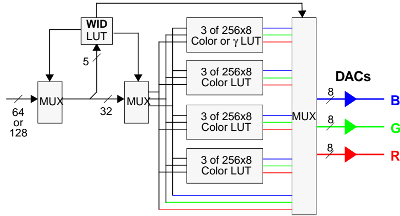
Figure 3-7 A functional diagram of the Bt497+ and Bt498+ RAMDACs
