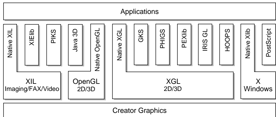
Figure 4-1 Solaris Foundation Graphics Libraries and layered interfaces
