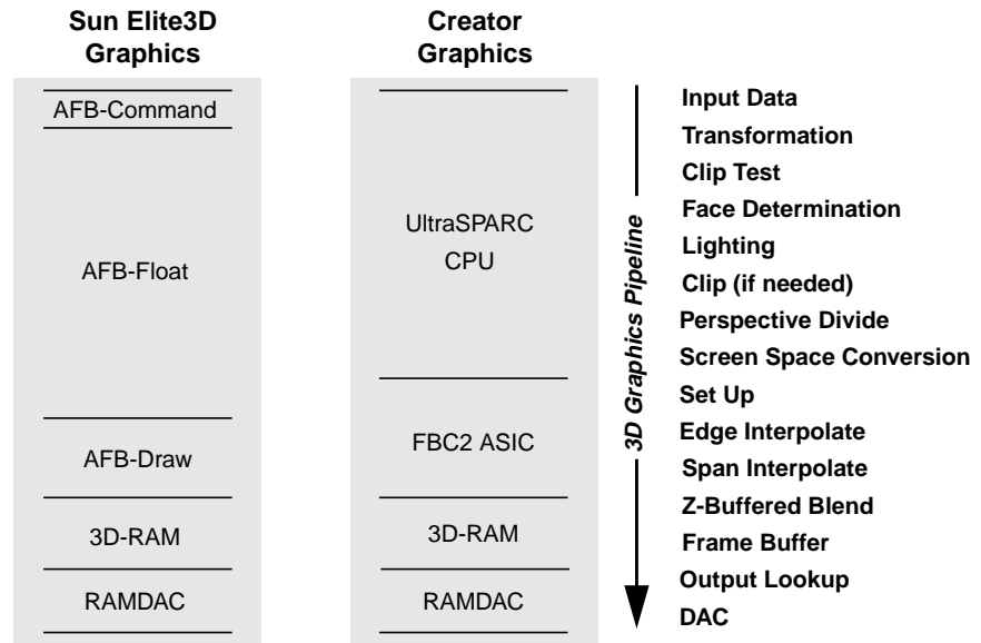
Figure 2-1 Pipeline differences between Sun's Elite3D and Creator Graphics systems
