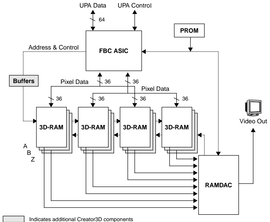
Figure 3-2 Combined Block diagram of Creator and Creator3D
