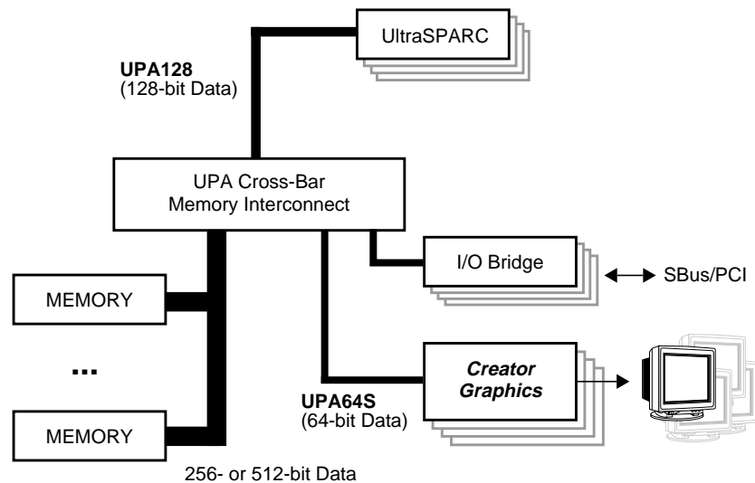
Figure 3-8 Creator Graphics block diagram
