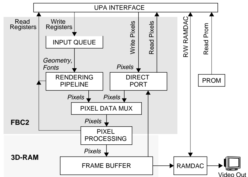
Figure 3-3 A logical view of the Creator Graphics subsystem
