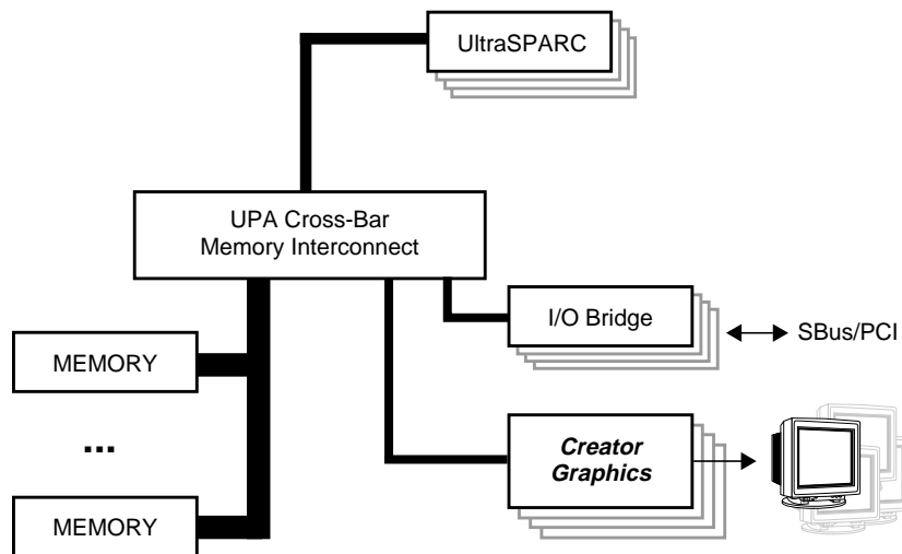
Figure 3-1 Creator Graphics system block diagram
