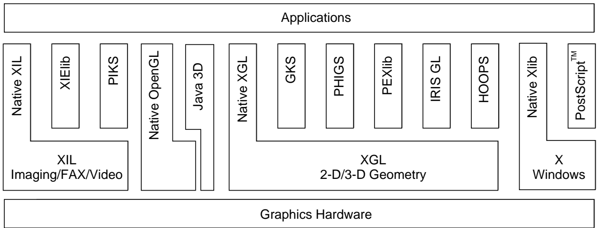
Figure 4. Graphics software interfaces
