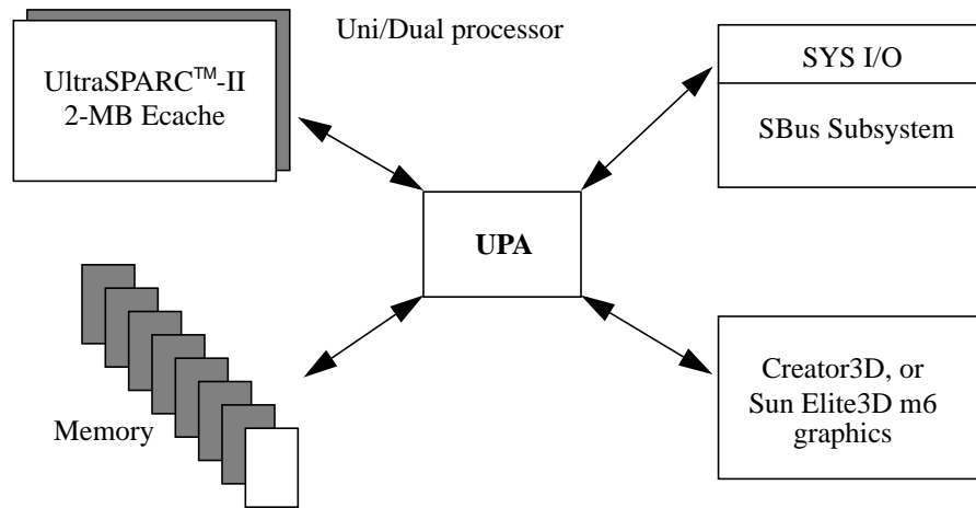
Figure 2. The Sun Ultra™ 2 workstation
